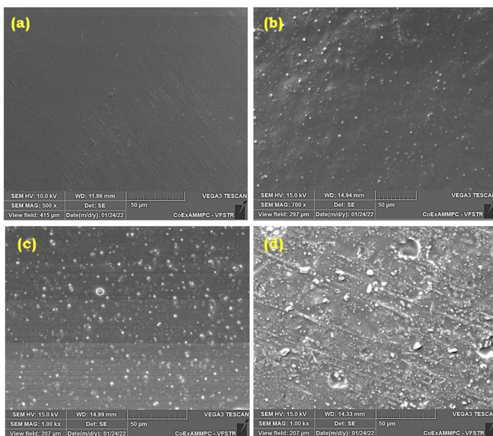
Fig. 6 SEM images of (a) poly[E-3ap] neat, (b) poly[E-3ap-co-SH(10%)]/BS 1 , (c) poly[E-3ap-co-SH(10%)]/BS 3 , and (d) poly[E-3ap-co-SH(10%)]/BS 5 .
